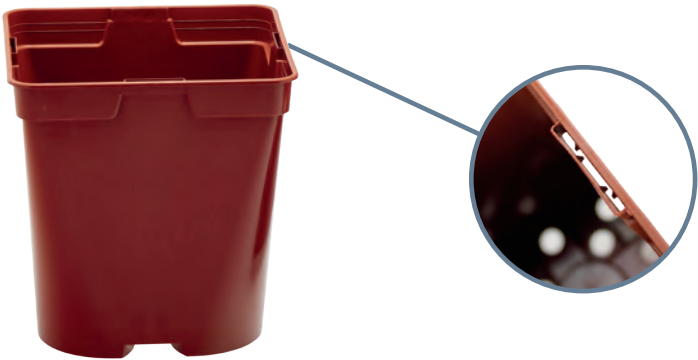
Bottom for sub-irrigation: Code 2209
